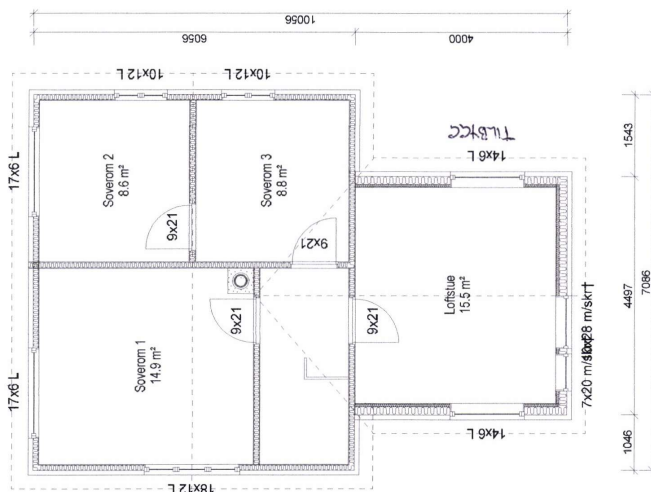
PLAN 2. ETG
