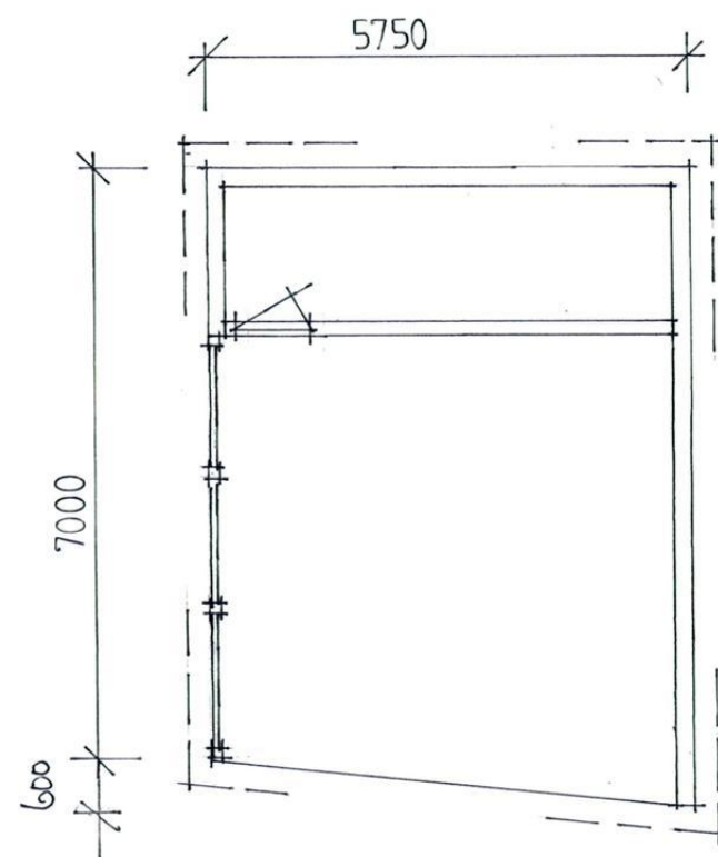
PLAN CARPORT
