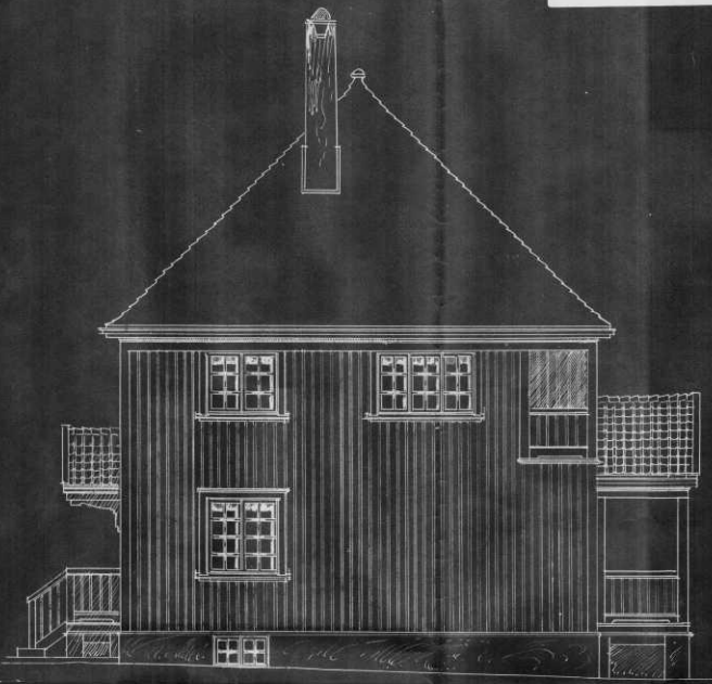
FACADE. MOT.
