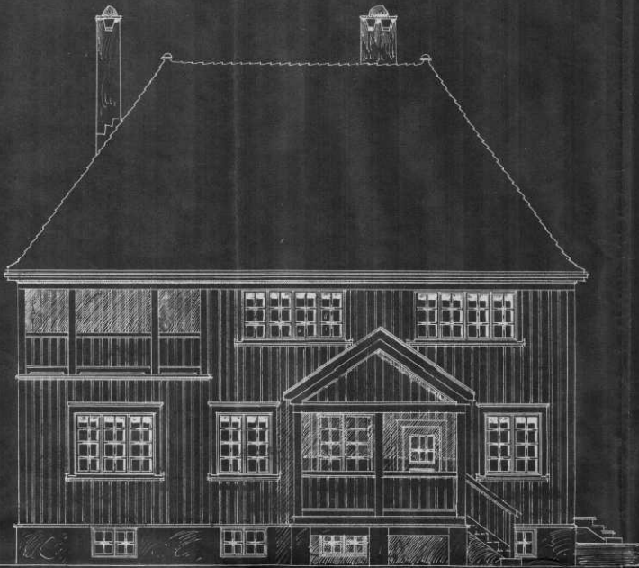
FACADE. MOT.
